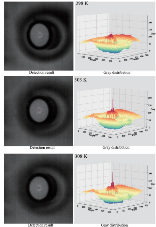
Fig. 3 Detection results and gray-scale distribution 图3 探测结果和灰度分布
