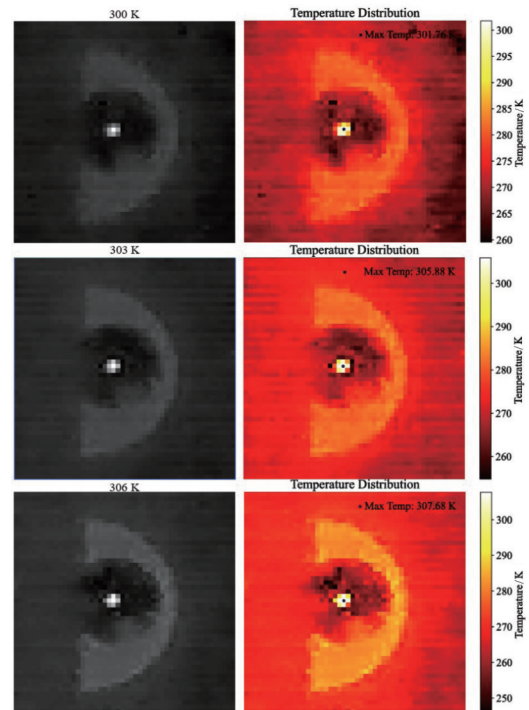
Fig. 8 Temperature field distribution
