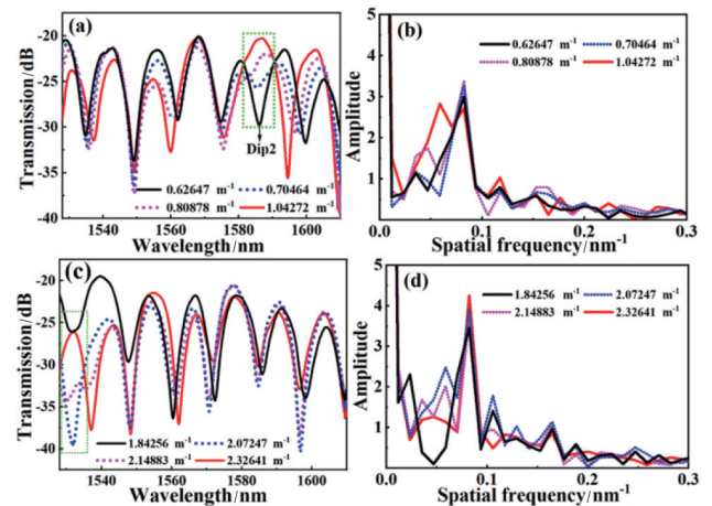
Fig. 7 (a) Transmission spectra with curvature range from 0.626 47 m -1 to 1.042 72 m -1 ; (b) the corresponding spatial frequency spectra; (c) transmission spectra with curvature range from 1.842 56 m -1 to 2.326 41 m -1 ; (d) the corresponding spatial frequency spectra 图7 (a)曲率在0.626 47~1.042 72 m -1 范围的透射光谱;(b)相应的空间频谱;(c)曲率在1.842 56~2.326 41 m -1 范围的透射光谱;(d)相应的空间频谱
