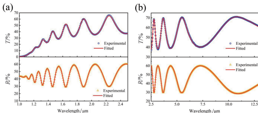
Fig. 3 Experimental (points) and fitted (lines) spectra of Ge film deposited at a rate of 1.0 nm/s in the (a) 1.0~2.5 \mu\text{m} and (b) 2.5~13.0 \mu\text{m} bands.
