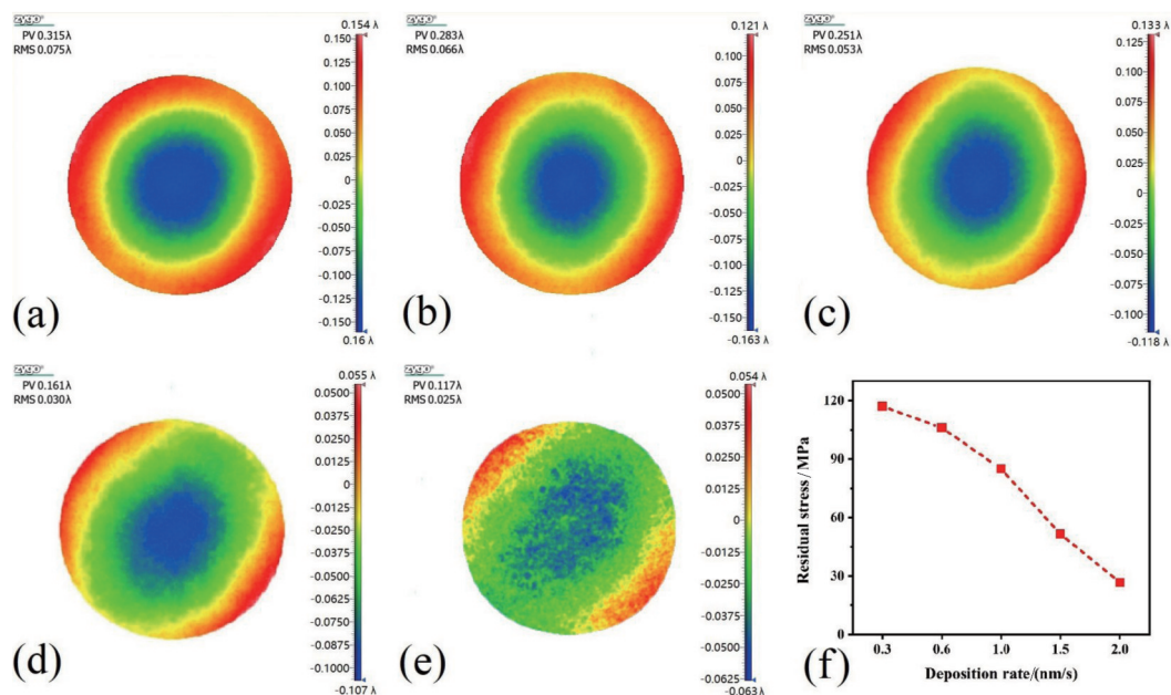
Fig. 6 Surface shapes of Ge film samples deposited at different rates: (a) 0.3 nm/s, (b) 0.6 nm/s, (c) 1.0 nm/s, (d) 1.5 nm/s, (e) 2.0 nm/s; (f) residual stresses of Ge film samples. 图6 不同速率沉积的Ge薄膜样品面形图:(a)0.3 nm/s,(b)0.6 nm/s,(c)1.0 nm/s,(d)1.5 nm/s,(e)2.0 nm/s;(f) Ge薄膜残余应力
