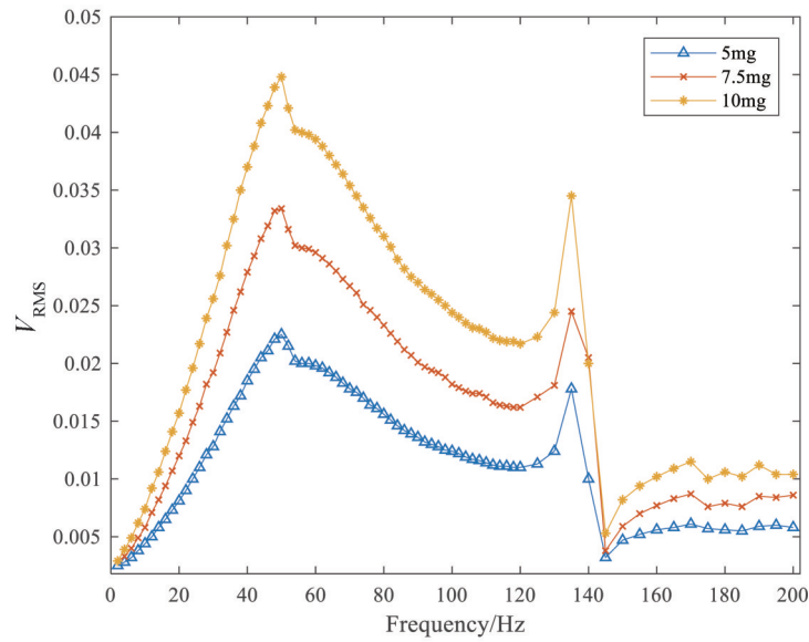
Fig. 9 The V_{RMS} of the moving mirror under 5 mg, 7.5 mg, and 10 mg sine excitation over 2-200 Hz 图9 5 mg, 7.5 mg, 10 mg 正弦激励下, 2~200 Hz 范围内动镜速度均方根值误差
