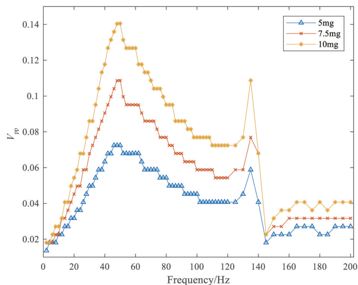
Fig. 8 The V_{pp} of the moving mirror under 5 mg, 7.5 mg, and 10 mg sine excitation over 2-200 Hz 图8 5 mg, 7.5 mg, 10 mg 正弦激励下, 2~200 Hz 范围内动镜速度峰峰值误差
