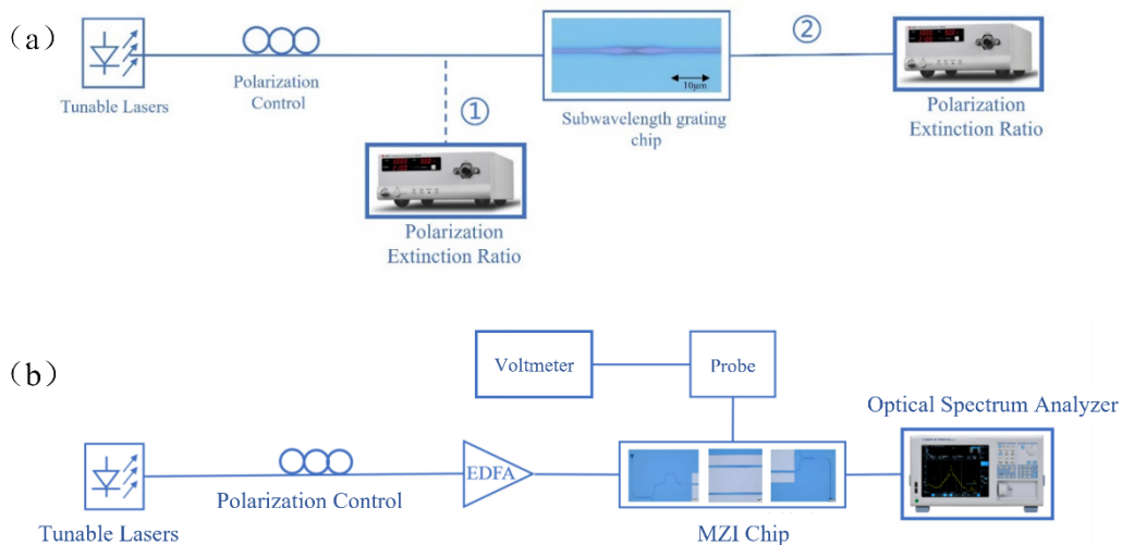
Fig. 7 (a) Polarization extinction ratio test system [18] ; (b) half-wave voltage test system
