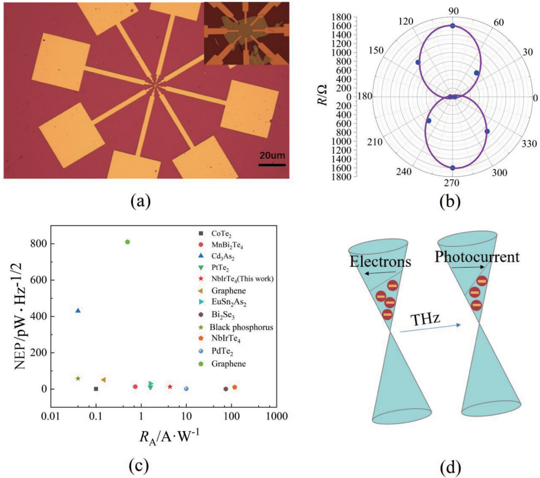
Fig. 6 Anisotropy of the device: (a) designed eight electrodes (the inset is an enlarged view of the intersection of the electrode and the material); (b) resistance values measured at every 45° angle (the maximum resistance ratio reaches 32); (c) comparison of responsivity and noise equivalent power with other detectors (The abscissa is displayed using log10 logarithmic coordinates); (d) schematic diagram of photocurrent generation of NbIrTe 4 .
