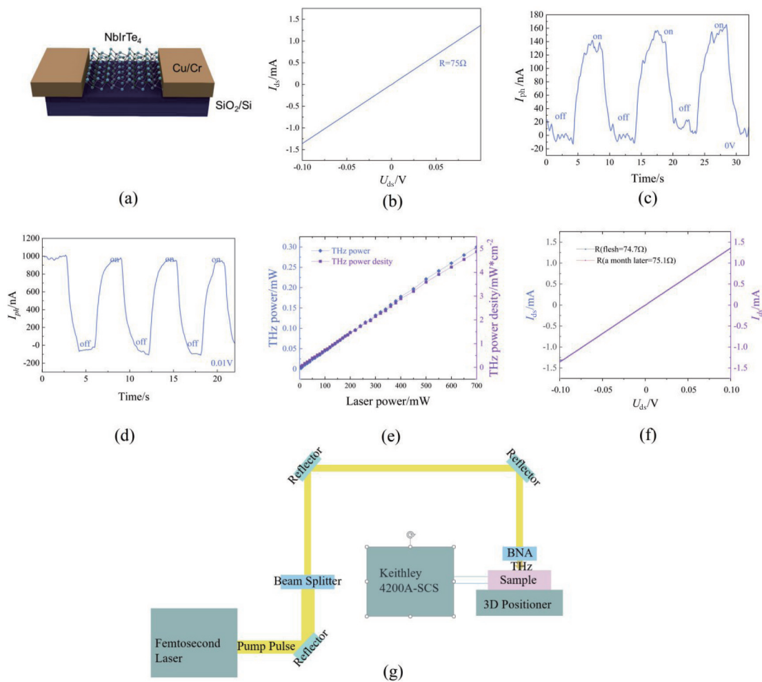
Fig. 5 Device measurement results: (a) schematic diagram of the detector; (b) electrical characteristics of the device; (c), (d) Terahertz response of the device under 0 bias and 0.01 V bias; (e) relationship between terahertz power and laser power; (f) the resistance change of the device after oxidation in air for one month; (g) schematic diagram of terahertz photoelectric response test system 图5 器件的测量结果:(a) 探测器的示意图;(b) 器件的电学特性;(c), (d) 器件在0偏压和0.01V偏压下的太赫兹响应;(e) 太赫兹功率和激光功率关系;(f) 器件在空气中氧化1个月的电阻变化;(g) 太赫兹光电响应测试系统
