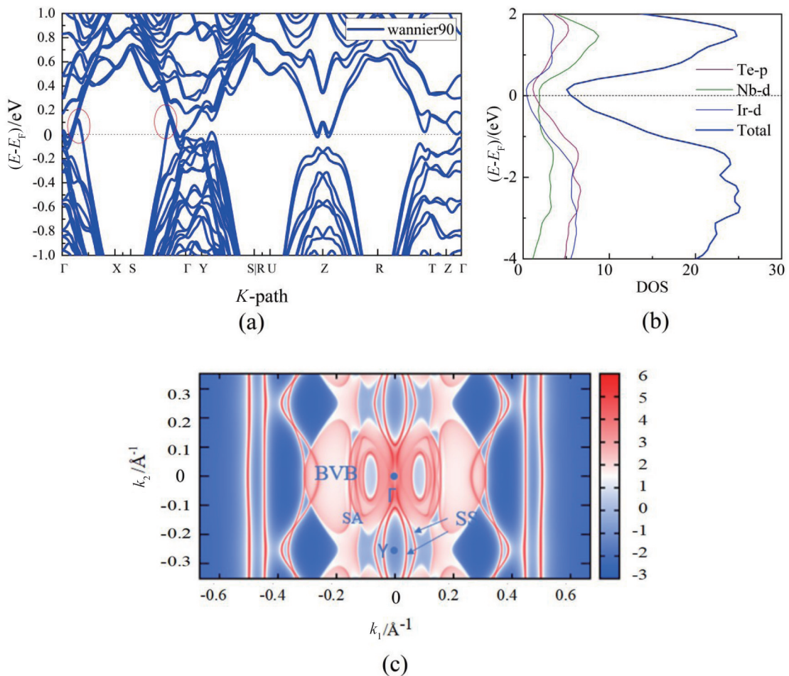
Fig. 2 Calculated band structure and surface states of NbIrTe 4 : (a) band structure of NbIrTe 4 (The red circles indicate the Weyl points of the material, and the dotted line indicates the Fermi surface); (b) density of states of NbIrTe 4 ; (c) calculated Fermi arc of NbIrTe 4 on the (001) surface
