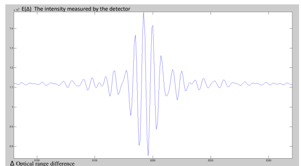
Fig. 6 Plot of test results of the planar angular mirror mechanism programme 图 6 基于角镜平动式干涉系统的测试结果图
