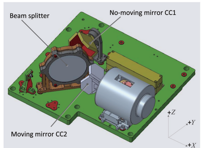
Fig. 3 Model of the interferometer
