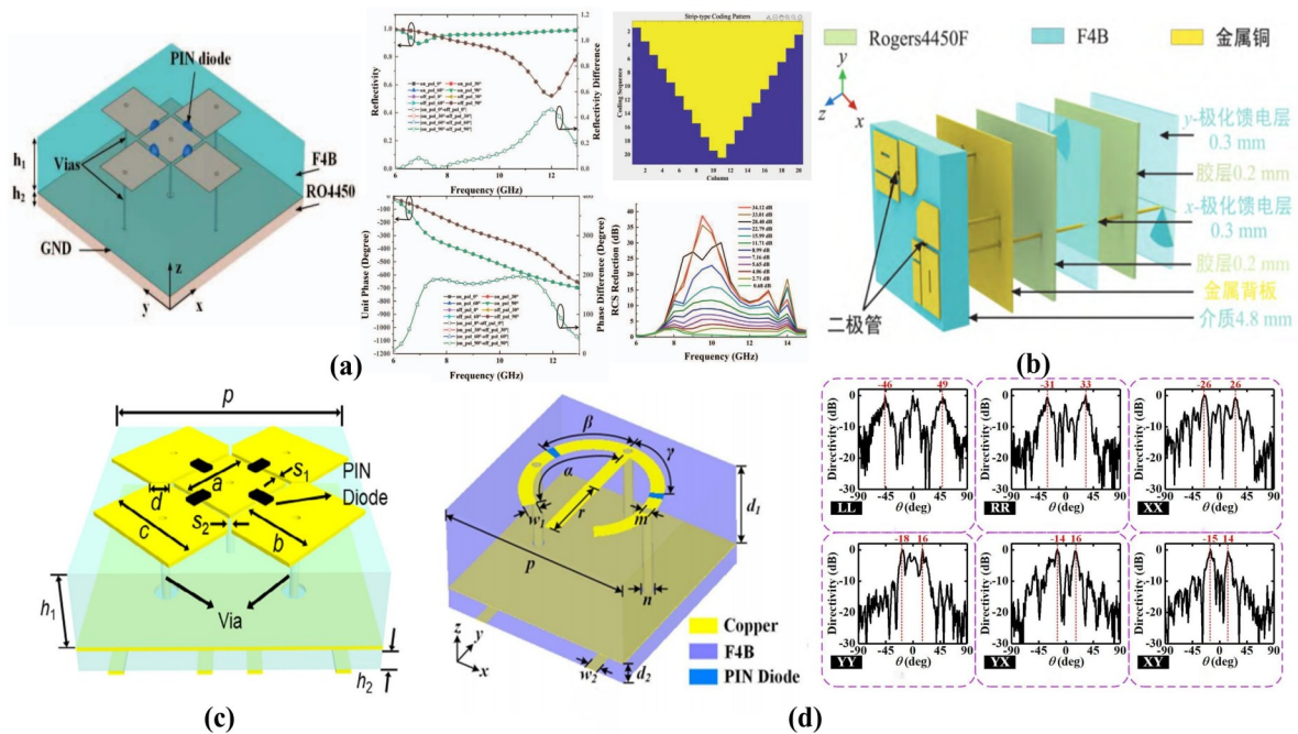
图6 (a) 双极化宽带超表面单元、单元反射率、单位相位差仿真结果、不同编码模式下的宽带可调谐RCS缩减的仿真结果 [83] ; (b) 1-bit 相位动态调控超表面单元 [84] ; (c) 45°对称超表面单元 [85] ; (d) 伞状超表面单元, 不同通道测试的归一化远场方向图 [86-87] Fig. 6 (a) Broadband dual polarized metasurface's meta-atom, the simulated results of unit cell reflectivity, unit phase and phase difference, the simulated results of wideband tunable RCS reduction with different coding patterns [83] ; (b) 1-bit phase modulation of metasurface's unit cell [84] ; (c) 45° symmetric metasurface's meta-atom [85] ; (d) umbrella shaped metasurface's meta-atom, the measured normalized far-field scattering patterns in different channels [86-87]
