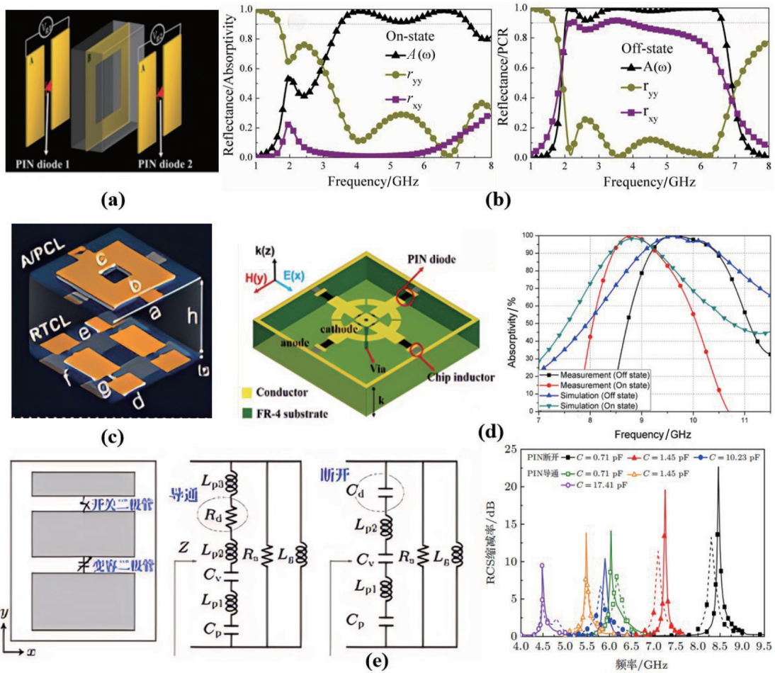
图4 (a)偏置电压如何独立应用的方案 [64] ; (b)所有的二极管都处于开启状态和所有二极管都处于关闭状态仿真结果 [65] ; (c)可重构超表面的示意图 [66] ; (d)吸波超表面单元形状,吸收率测量和仿真结果 [67] ; (e)超宽带有源超表面单元,开关导通及断开时的等效电路模型,仿真与实测的 RCS 减缩曲线 (实线, 仿真结果; 虚线, 实测结果) [71-72] Fig. 4 (a) Scheme of how the bias voltages are applied independently [64] ; (b) simulation results for all the diodes are in on-state and all the diodes are in off-state [65] ; (c) the sketch of the proposed reconfigurable metasurface [66] ; (d) geometry of the proposed absorber unit cell, measured and simulated absorptivity of the proposed absorber [67] ; (e) ultra-wideband active metasurface absorber, equivalent circuit model of PIN diode at ON state and OFF state, simulated and measured monostatic RCS reduction. (Solid lines, simulated results; dashed lines, measured results) [71-72]
