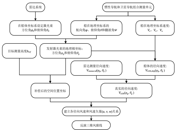
图3 船载大气多参数探测激光雷达数据姿态校正和风速反演流程图 Fig. 3 Flow chart for attitude correction and inversion for data detected by shipborne multi-parameter atmospheric lidar
