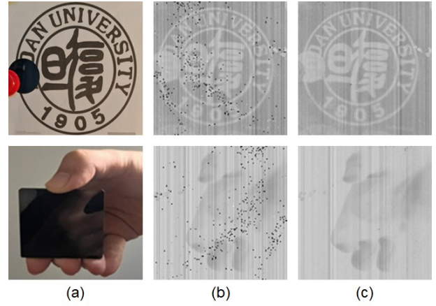
Fig. 6 This set of images demonstrates the model's processing effect on images actually captured by the PbS focal plane detector: (a) is a real photograph taken by the camera, with black circular and square shapes representing silicon wafers; (b) is the near-infrared image captured by the PbS focal plane detector; (c) is the final processed image by the model
