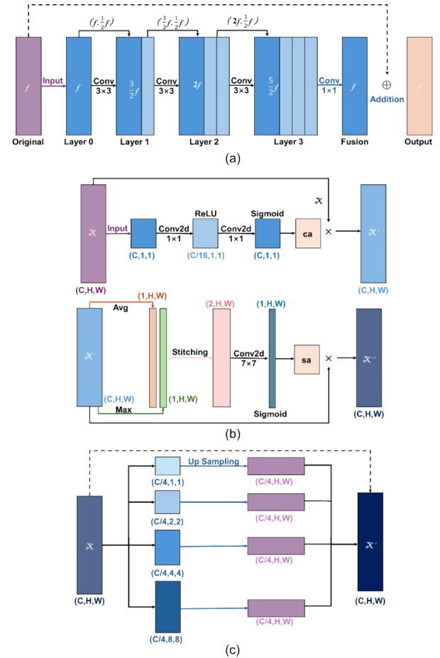
Fig. 4 (a) is the schematic diagram of the Residual Dense Fusion Block process; (b) is the schematic diagram of the Dual Attention mechanism, and (c) is the schematic diagram of the Pyramid Pooling module
