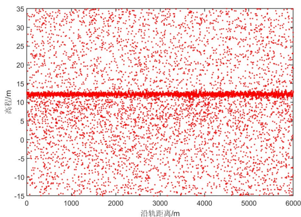
图1 ATL03数据可视化之后的点云图,红点表示ATLAS探测到的光子事件,横坐标表示获取的光子对应的沿轨距离,纵坐标是根据获取的光子对应飞行时间计算得到的高程值 Fig. 1 Point cloud diagram by visualizing ATL03 data, the red dots represent photon events detected by the ATLAS, with the horizontal coordinate indicating the along-track distance corresponding to the acquired photon, and the vertical coordinate denoting the elevation value derived from the time-of-flight of the detected photon
