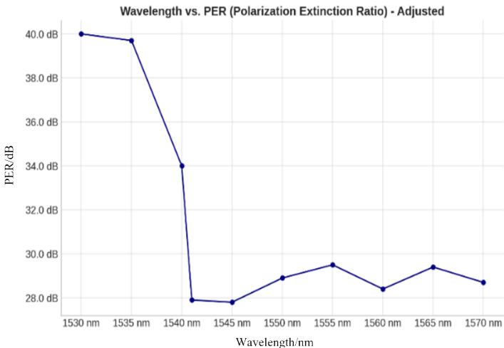
Fig. 8 Wavelength and extinction ratio test data 图8 波长及消光比测试数据
