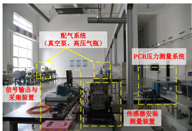
图6 激波管实验系统照片 Fig. 6 Photograph of shock tube experimental system
