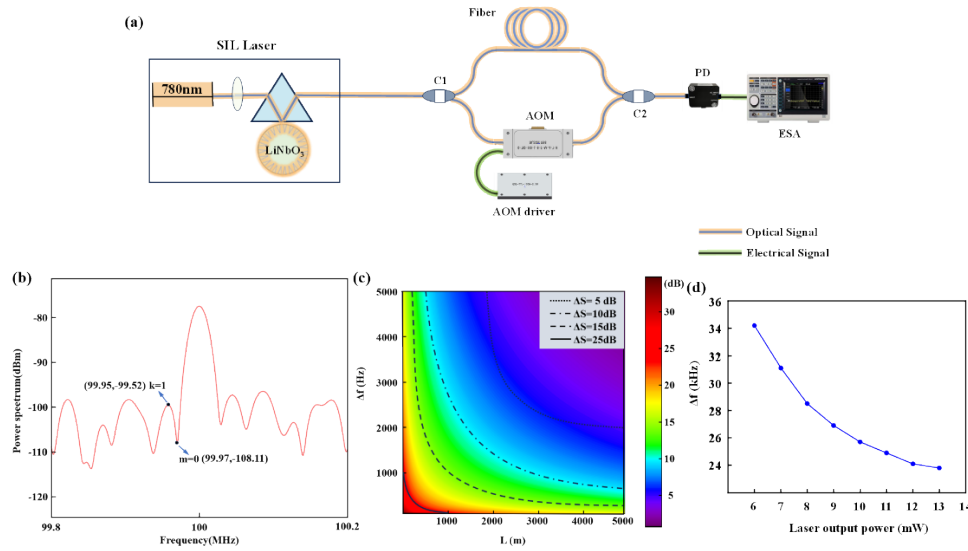
Fig. 4 Measured laser linewidth for the short delayed self-heterodyne interferometry. (a) C1 and C2: optocoupler (50/50). The delayed fiber length is 150 m. PD: photoelectric detector. AOM: acousto-optic modulator (100 MHz). ESA: electronic spectrum analyzer. (b) Plot of the envelope data for the delayed fiber length of 150 m used. (c) Magnitude difference between a pair of extreme points corresponding to different delayed fiber lengths ( L ) and laser linewidth ( \Delta f ). (d) Laser linewidth corresponding to different laser power 图4 短光纤延迟自外差法的测激光线宽。(a) C1和C2:光耦合器(50/50)。延迟光纤长度为150米。PD:光电探测器。AOM:声光调制器(100MHz)。ESA:电子频谱分析仪。(b)使用的延迟光纤长度为150米的包络数据图。(c)不同延迟光纤长度( L )和激光线宽( \Delta f )所对应的一对极值点的幅度差。(d)不同的激光器功率对应的激光线宽
