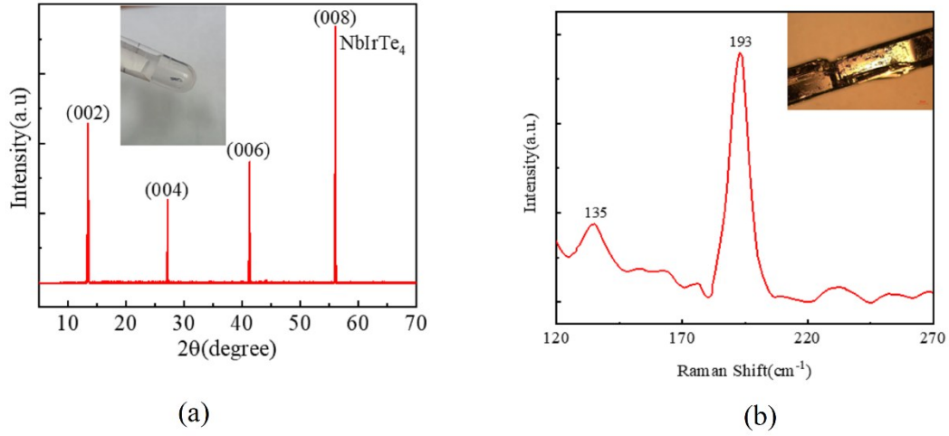
Fig. 3 Characterization of NbIrTe 4 . (a) XRD characterization of NbIrTe 4 , with high peaks, narrow half-wave width and almost no impurity peaks. The inset is a well-grown NbIrTe 4 crystal. (b) Raman characterization of NbIrTe 4 . The inset is a NbIrTe 4 crystal photographed with a microscope.
