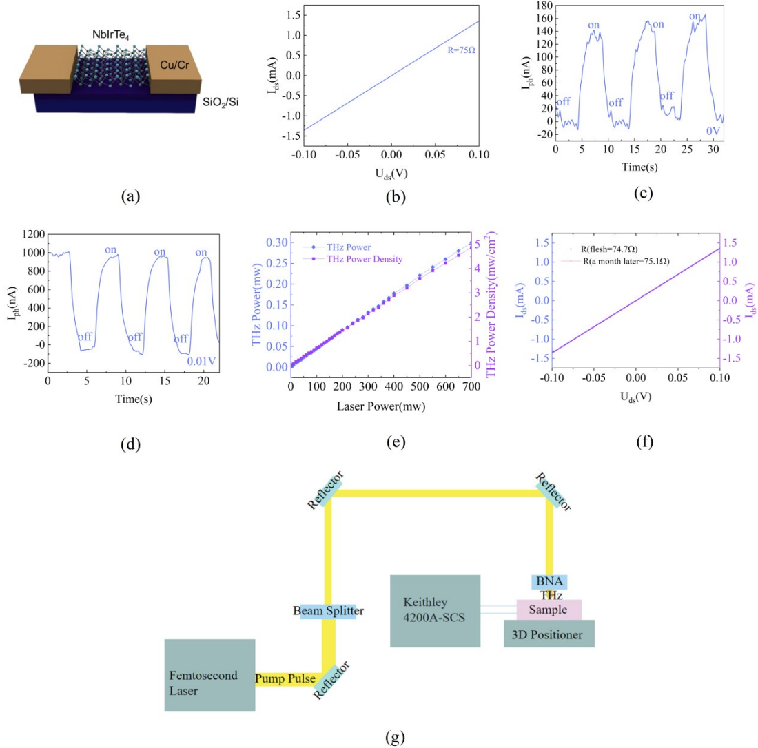
Fig. 5 Device measurement results. (a) Schematic diagram of the detector. (b) Electrical characteristics of the device. (c), (d) Terahertz response of the device under 0 bias and 0.01V bias. (e) Relationship between terahertz power and laser power. (f) The resistance change of the device after oxidation in air for one month. (g) Schematic diagram of terahertz photoelectric response test.
