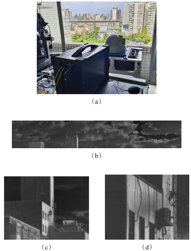
Fig. 17 Outfield imaging of infrared search and track: (a) out-field imaging; (b) panoramic search imaging diagram; (c) coarse track imaging diagram; (d) fine track imaging diagram 图 17 红外搜跟外场成像: (a) 外场成像; (b) 全景搜索成像图; (c) 粗跟踪成像图; (d) 精跟踪成像图
