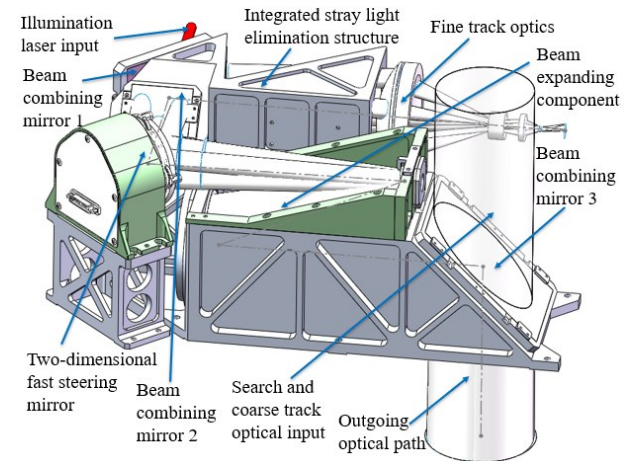
Fig. 8 Search and track opto-mechanical beam combining schematic diagram 图8 搜跟光机合束示意图
