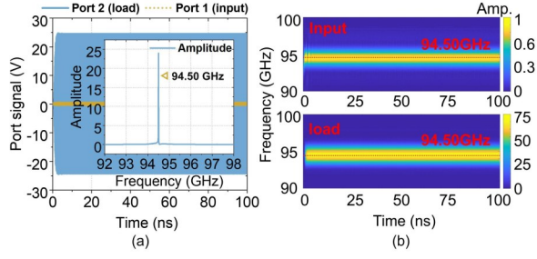
Fig. 5 (a) The amplitude and spectrum for the input and load signals, and (b) the corresponding time-frequency analysis diagrams.
