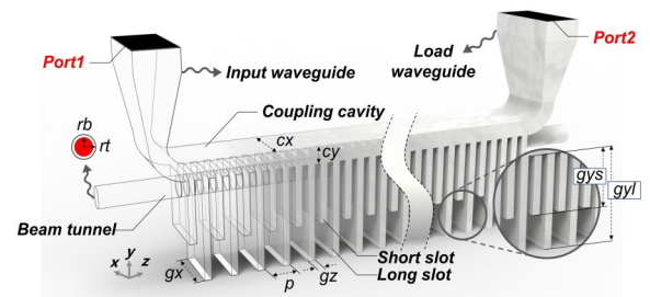
Fig. 2 The three-dimensional schematic diagram of the broadband input cavity.
