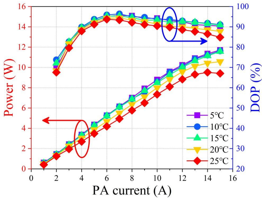
图 6 MOPA 器件的功率和偏振度随热沉温度的变化: Figure (6) The impact of heat sink temperature on the power and DOP of MOPA device
