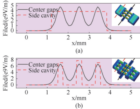
Fig. 3 Axial field distribution at center gaps and side cavities of two different cavities, (a) the traditional ladder type cavity, (b) the novel cavity
