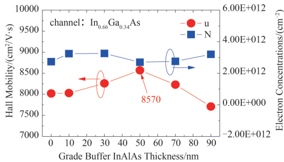
Fig. 5 Hall mobility and electron concentrations in different InAlAs graded buffer layer thickness 图5 不同厚度 InAlAs 渐变缓冲层霍尔迁移率和电子密度
