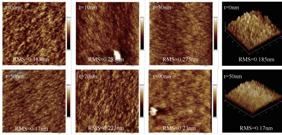
Fig. 4 The surface morphology of the InGaAs channel with different InAlAs graded buffer layer thickness 图4 带不同厚度 InAlAs 渐变缓冲层的 InGaAs 的表面形貌
