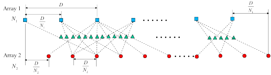
Fig. 2 Diagram of MIMO linear array configuration adopted by the proposed new MIMO mechanism 图 2 新型 MIMO 体制线性天线阵列配置示意图
