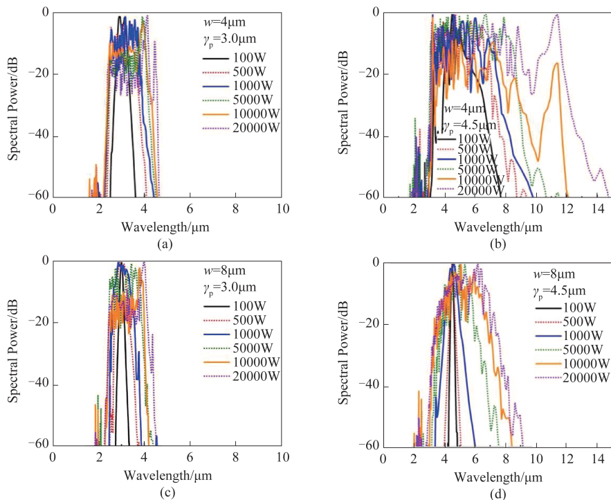
Fig. 5 Simulated SC spectra at a pump wavelength of (a) 3.0\mu\text{m} , (b) 4.5\mu\text{m} , (c) 3.0\mu\text{m} and (d) 4.5\mu\text{m} for the two waveguides at different peak power up to 20\text{ kW} , respectively.
