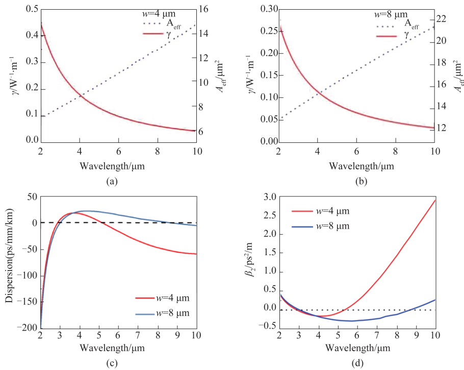
Fig. 4 Effective area and nonlinear coefficient of the fundamental mode calculated in the waveguides (a) w = 4\mu\text{m} , H_1 = 2\mu\text{m} , and H_2 = 1\mu\text{m} (b) w = 8\mu\text{m} , H_1 = 2\mu\text{m} , and H_2 = 1\mu\text{m} . (c) Dispersion distribution of the waveguides with w = 4 and 8\mu\text{m} . (d) The second-order dispersion of the waveguides with w = 4 and 8\mu\text{m} .
