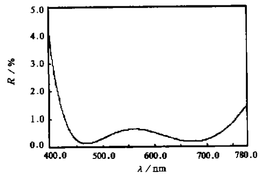
图 5 经折射率补偿矫正过的宽带 8 层增透膜的反射光谱实测曲线 Fig. 5 The measured reflection curve of a broad-band eight-layer anti-reflection coating corrected by compensation of refractive index
