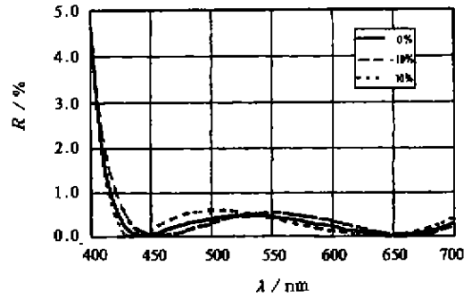
图 4 第 5 层膜的厚度变化对反射曲线的影响 Fig. 4 Influence of change of the 5th layer thickness on the reflection curve
