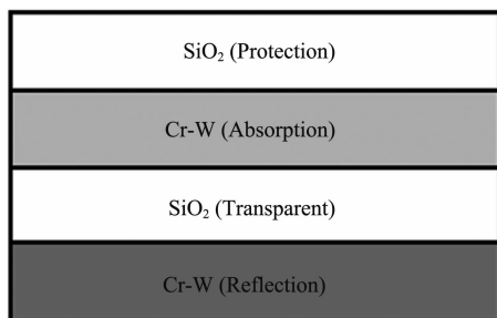
Fig. 4 Schematic structure of newly designed 4-layer alloy/dielectric device consisting of [ \text{SiO}_2/\text{Cr-W}/\text{SiO}_2/\text{Cr-W} ]
