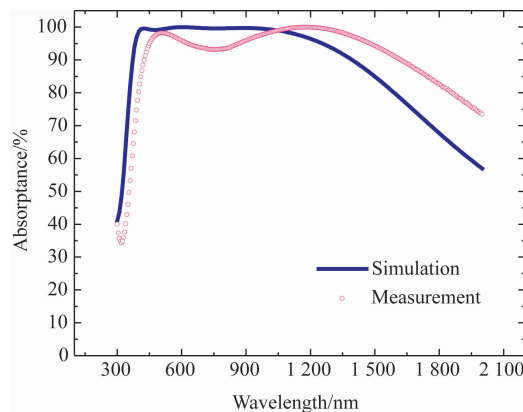
Fig. 6 Tested and calculated absorption of newly designed 4-layer alloy/dielectric device consisting of [ \text{SiO}_2/\text{Cr}/\text{SiO}_2/\text{CrW} 33:67]
