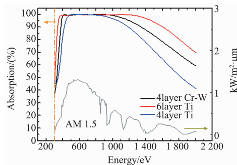
Fig. 5 Black line is the simulated absorption spectrum for 4-layer structure [ \text{SiO}_2 90.7 nm/Cr 5.2 nm/ \text{SiO}_2 93.4 nm/ CrW33:67 >200 nm]. The absorption spectra of the early designed 4 and 6-layer structures are also presented in comparison
