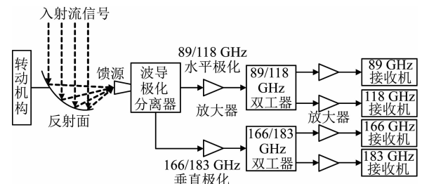
图 3 基于双工器和波导极化分离器的分频技术 Fig. 3 Frequency separation technique based on duplexers and waveguide polarization separators
