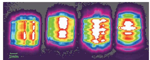
Fig. 7 The mid-infrared camera image of the total beam spot in near field
