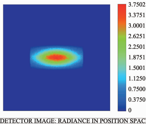
Fig. 2 The collimated beam spot in near field of single diode laser by simulation 图 2 单管二极管激光器近场准直光斑的模拟结果
