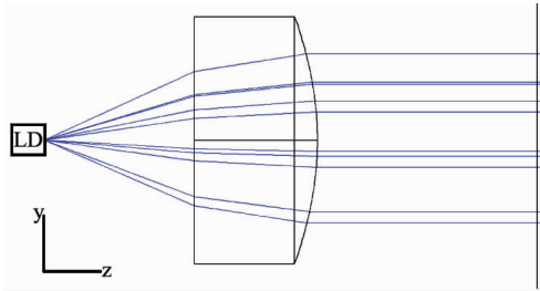
Fig. 1 The collimation design of single laser diode (LD) 图 1 单管激光二极管准直设计图
