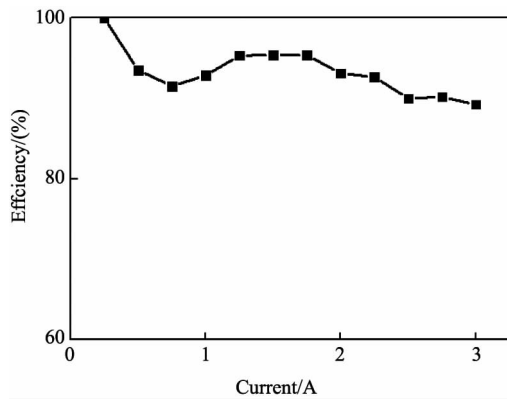
Fig. 9 The efficiency of beam shaping versus driving current 图9 光束整形效率随驱动电流变化图
