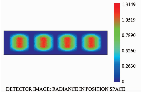
Fig. 6 The total beam spot in near field of the beam shaping system by simulation
