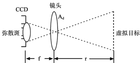
图3 模拟目标的成像示意图 Fig. 3 Imaging schematic diagram of the simulated target
