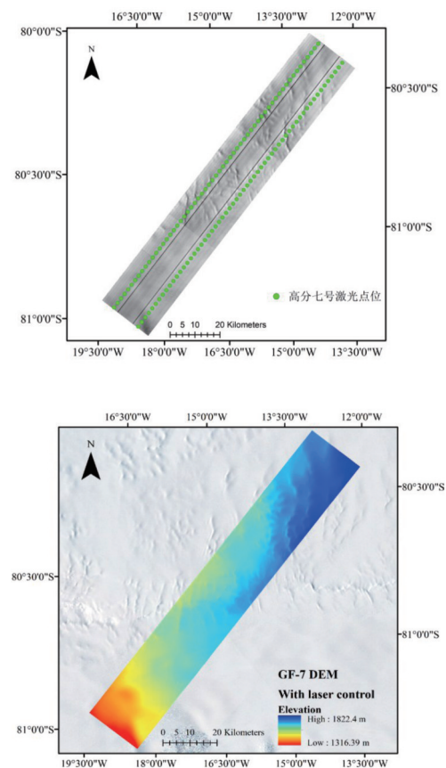
图5 南极区域GF-7卫星立体影像及激光测高数据 Fig. 5 GF-7 satellite stereo images and laser altimeter in the Antarctic
