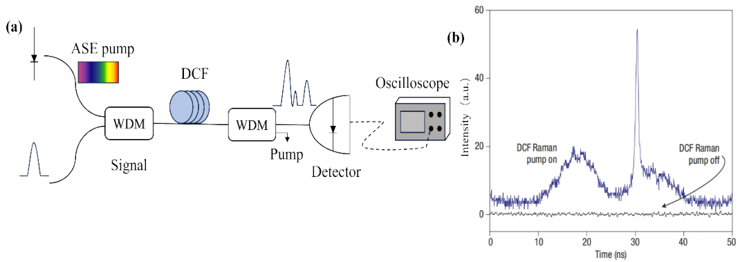
图3 光谱学中放大波长-时间变换的演示。(a)放大波长-时间变换结构示意图;(b)输出结果图。图片引用自文献[18] Fig. 3 Demonstration of amplified wavelength-time conversion in spectroscopy. (a) schematic of the amplified wavelength-time conversion structure; (b) output-result diagram. The pictures are quoted from Ref. [18]
