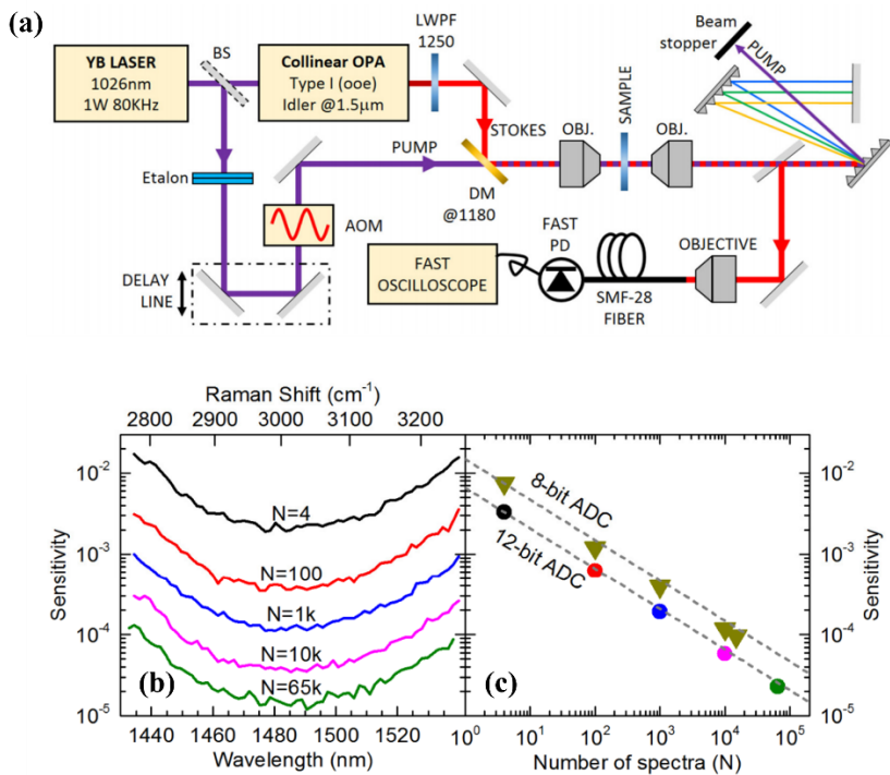
图4 (a)实验装置示意图;(b)用12位示波器测量下的不同光谱数量下SRG的波长相关均方根值和灵敏度;(c)对于8位和12位示波器,SRG的光谱数量与灵敏度函数关系。图片引用自文献[19] Fig. 4 (a) Schematic of the experimental setup; (b) Wavelength-dependent RMS values and sensitivities of SRG at different spectral numbers measured using a 12-bit oscilloscope; (c) Spectral number of SRG as a function of sensitivity for 8-bit and 12-bit oscilloscopes. The pictures are quoted from Ref. [19]
