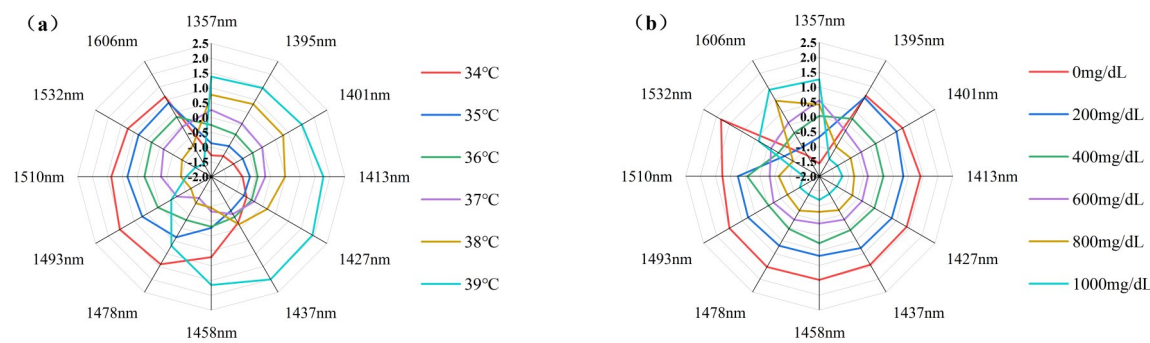
图4 不同温度与葡萄糖浓度组织仿体溶液的雷达图:(a)不同温度;(b)不同糖浓度 Fig. 4 Radar charts of tissue phantom solutions under different temperatures and glucose concentrations: (a)different temperatures; (b)different glucose concentrations
