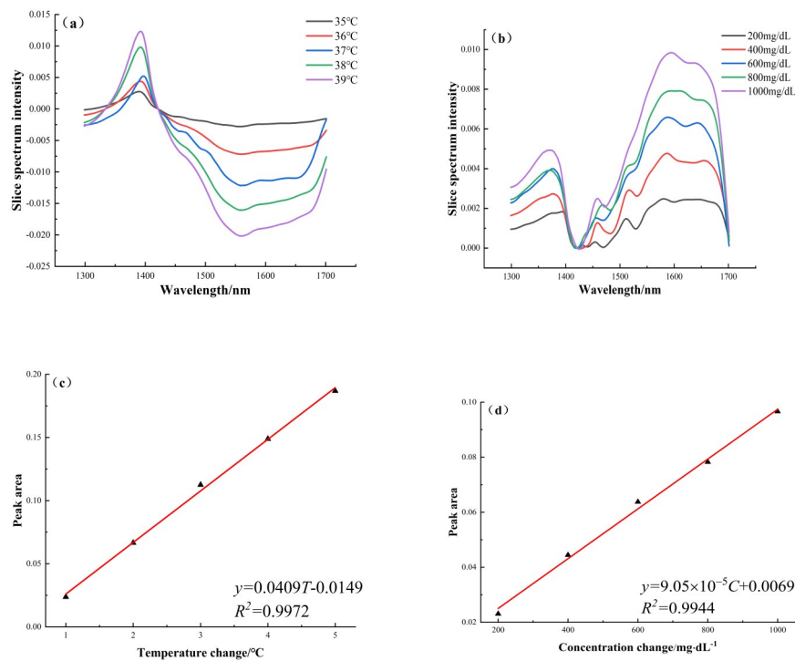
图5 不同条件下2T2D-COS异步谱1 420 nm处的切片谱及与1 595~1 605 nm波段强度的拟合关系:(a)不同温度下切片谱;(b)不同糖浓度下切片谱;(c)切片谱强度与温度变化量的拟合关系;(d)切片谱强度与糖浓度变化量的拟合关系 Fig. 5 The slice spectrum at 1 420 nm of 2T2D-COS asynchronous spectra under different conditions and their fitting relationship within 1 595~1 605 nm band intensities: (a)the slice spectrum under different temperatures; (b)the slice spectrum under different glucose concentrations; (c)the fitting relationship between the slice spectrum intensity and the temperature variation; (d)the fitting relationship between the slice spectrum intensity and the glucose concentration variation
