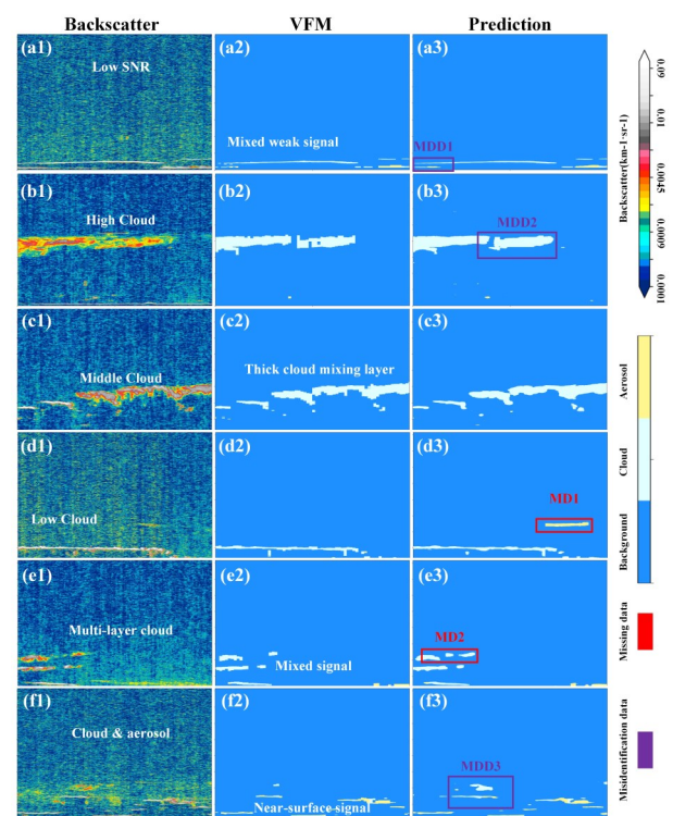
图4 案例分析,低信噪比下的层次识别结果:(a1~3);不同情形云层次识别结果:(b1~3)高云,(c1~3)中云,(d1~3)低云,(e1~3)多层云;不同情形云-气溶胶混合时的层次识别结果:(f1~3) Fig. 4 Case analysis, hierarchical recognition results under low signal-to-noise ratio: (a1-3); cloud hierarchical recognition results in different scenarios: (b1-3) high cloud, (c1-3) middle cloud, (d1-3) low cloud, (e1-3) multi-layer cloud; hierarchical recognition results for cloud-aerosol mixtures in different scenarios: (f1-3)
