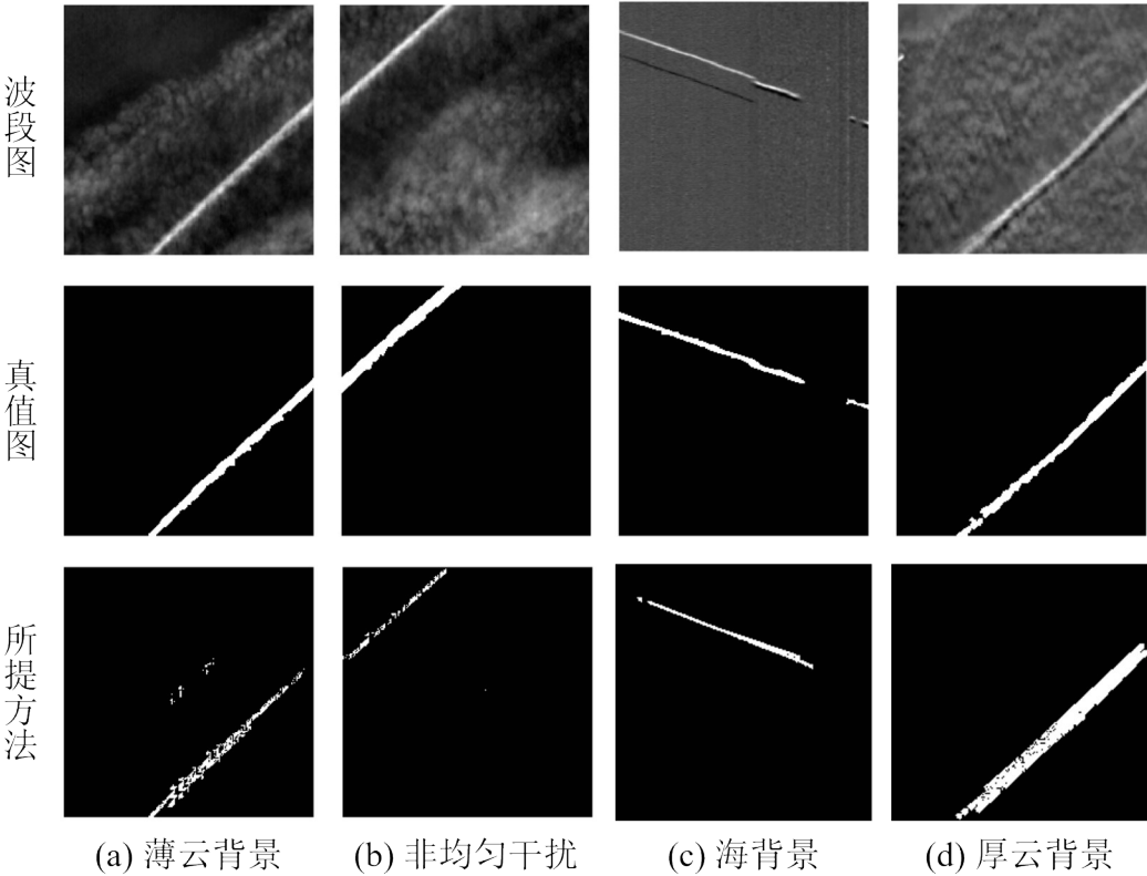
图 8 所提方法在 GF-5 SWIR 图像的实验结果: (a)Scene 1: GF-5 SWIR (薄云背景). (b) Sence 2: GF-5 SWIR(非均匀性干扰). (c) Sence 3: GF-5 SWIR(海背景). (d) Sence 4: GF-5 SWIR(厚云背景) Fig. 8 Experimental results of the proposed method on GF-5 SWIR images: (a) Scene 1: GF-5 SWIR (thin cloud background). (b) Scene 2: GF-5 SWIR (non-uniform interference). (c) Scene 3: GF-5 SWIR (sea background). (d) Scene 4: GF-5 SWIR (thick cloud background)
