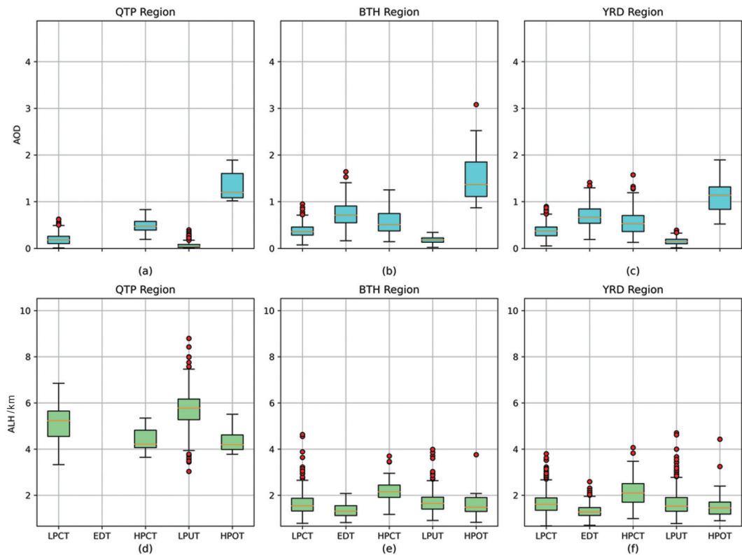
图9 五种剖面在典型地域上的分布:(a~c)AOD分布;(d~f)ALH分布 Fig. 9 The distribution for the five profiles in typical regions: (a-c) AOD distribution; (d-f) ALH distribution
