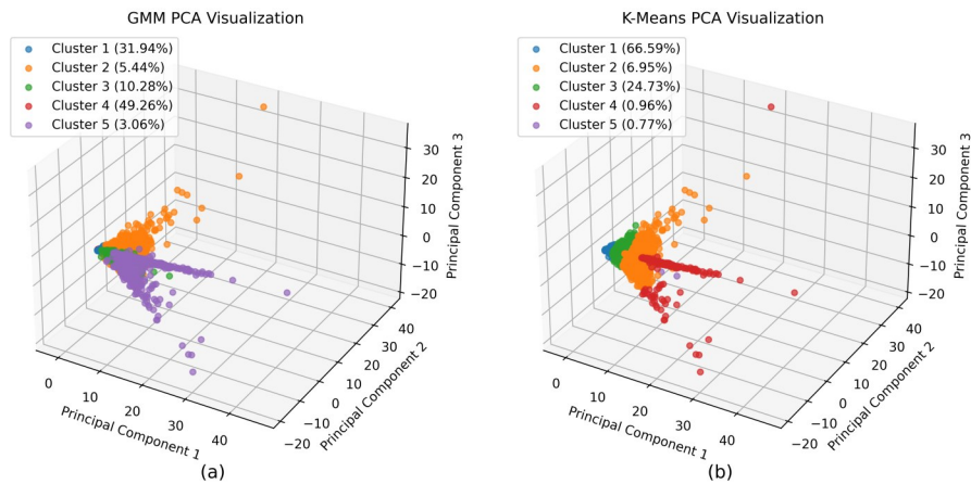
图3 经过PCA处理后的聚类方法的三维可视化数据图:(a)GMM;(b)K-means Fig. 3 Three-dimensional visualization of clustering methods after PCA processing: (a) for GMM; (b) for K-means
