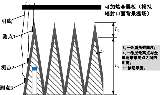
图10 定标源涂层表面温梯的薄膜铂电阻贴敷方案 Fig. 10 Thin PRT measurement upon the surface of coating layers of MCT.
