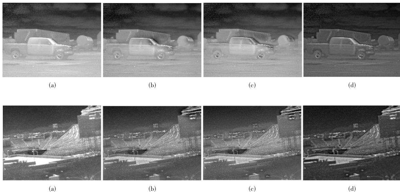
图 15 串联式融合算法对比:(a)文献[53]; (b)NSCT; (c)NSST; (d)NSST-Tophat; (e)文献[53]; (f)NSCT; (g)NSST; (h)NSST-Tophat
