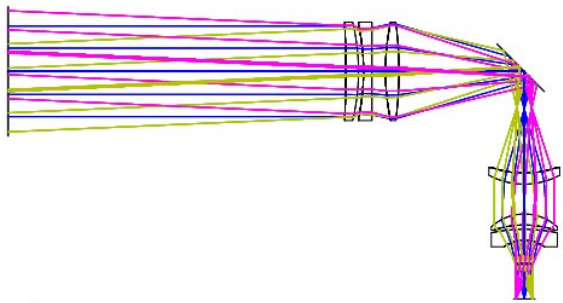
Fig. 10 Search and coarse track module optical path diagram 图10 搜索及粗跟踪模块光路图
