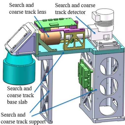
Fig. 9 Opto-mechanical structure of search and coarse track module 图9 搜索及粗跟踪模块光机结构
