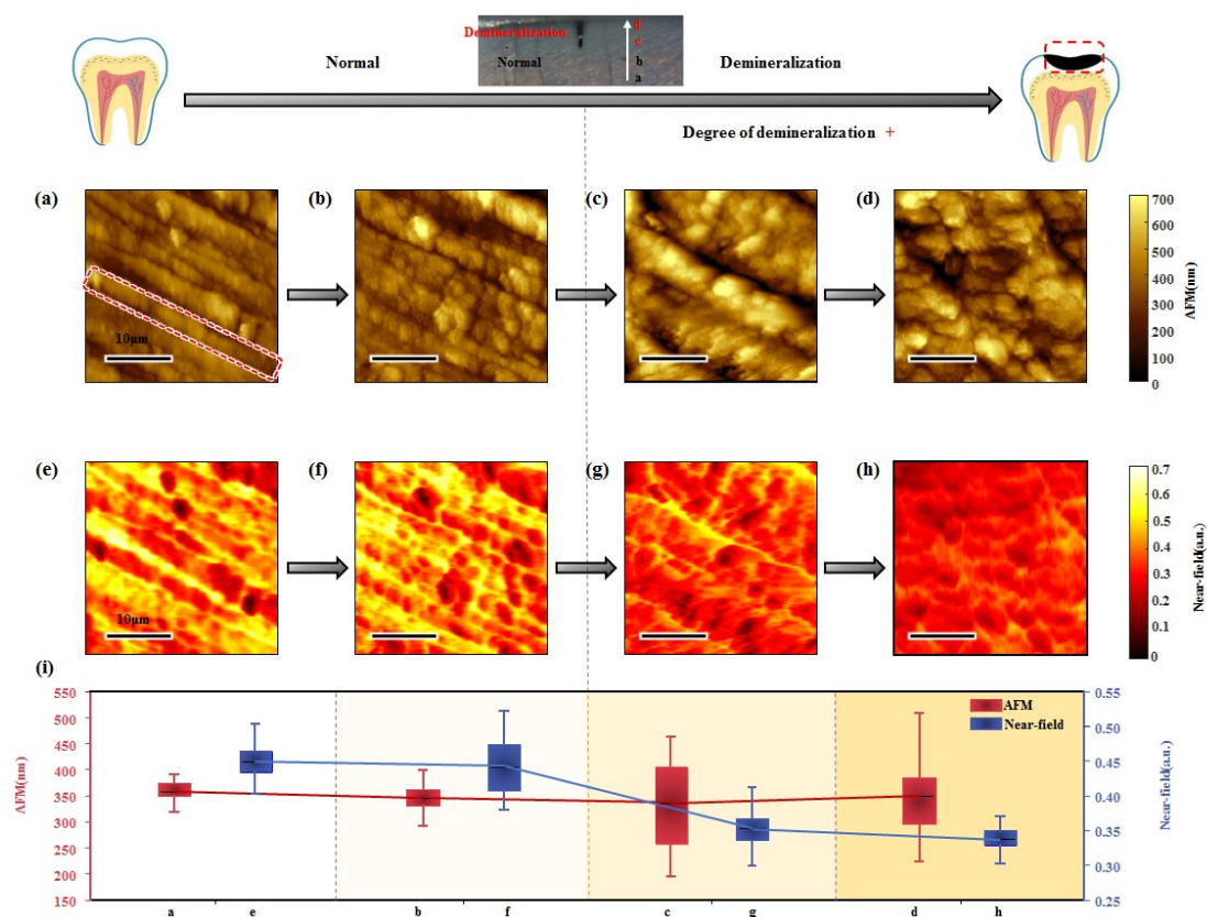
Fig. 3 AFM and near-field imaging results: (a)–(d) AFM results; (e)–(h) Near-field imaging results; (i) The boxplot of AFM and near-field data in each region. The black line in each box represents the mean value which is connected to form the mean value line
