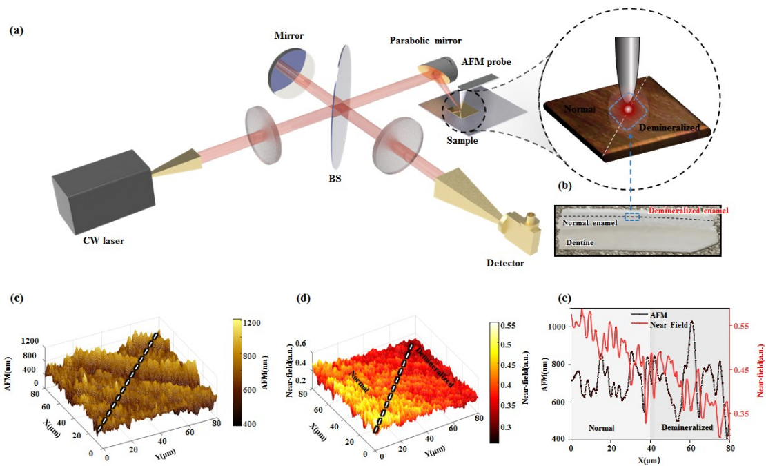
Fig. 1 Near-field imaging system and results; (a) Schematic illustration of the CW THz-SNOM setup; (b) Photo of the tooth slice (the area highlighted by the blue curve is the scanning range); (c) AFM results; (d) Near-field imaging results; (e) AFM and near-field signals along the dashed line 图1 近场成像系统和结果:(a)连续波近场系统图;(b)牙齿切片光学图片(蓝色曲线框住区域为扫描区域);(c)AFM成像结果;(d)近场成像结果;(e)沿虚线处的AFM和近场数据
