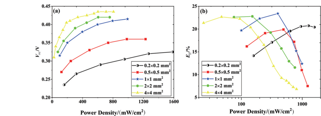
图7 不同器件区面积的激光光伏电池的性能参数随入射光功率密度的变化:(a)开路电压;(b)转换效率 Fig. 7 Performance parameters of laser photovoltaic cells with different cell areas versus the incident power density: (a) open-circuit voltage; (b) conversion efficiency
