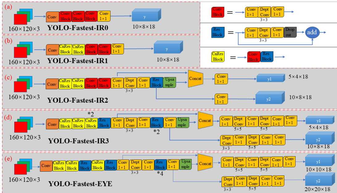
Fig. 2 The YOLO-Fastest-IR network structures with four different levels of complexity
