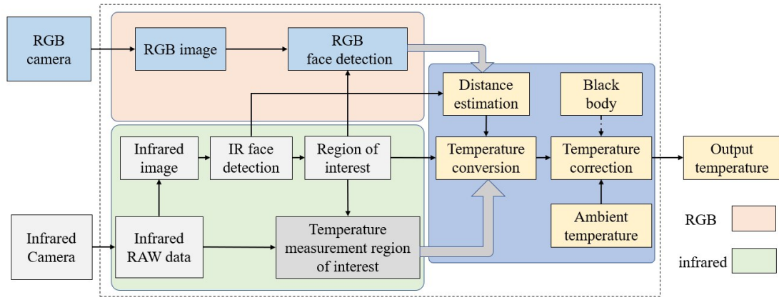
Fig. 1 The procedure of the working process of the dual band ITC system
