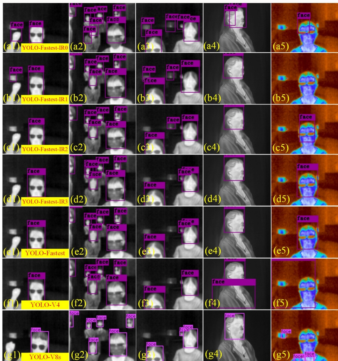
Fig. 4 The comparative and generalization experiments of different models: (a1~a5) the detection effect of YOLO-Fastest-IR0; (b1~b5) the detection effect of YOLO-Fastest-IR1; (c1~c5) the detection effect of YOLO-Fastest-IR2; (d1~d5) the detection effect of YOLO-Fastest-IR3; (e1~e5) the detection effect of YOLO-Fastest; (f1~f5) the detection effect of YOLO-V4; (g1~g5) the detection effect of YOLO-V8s
