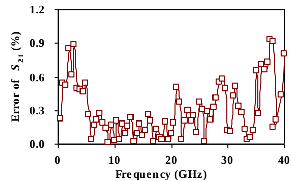
(b) S_{21}
