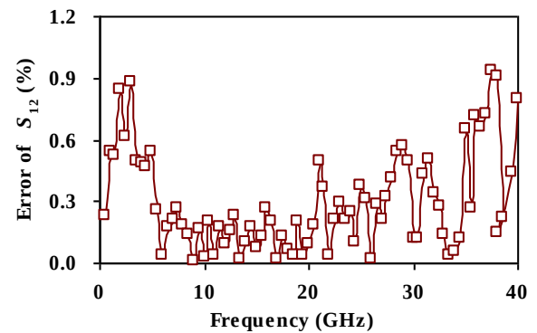
(c) S_{12}
