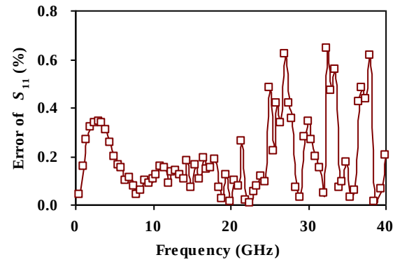
(a) S_{11}
