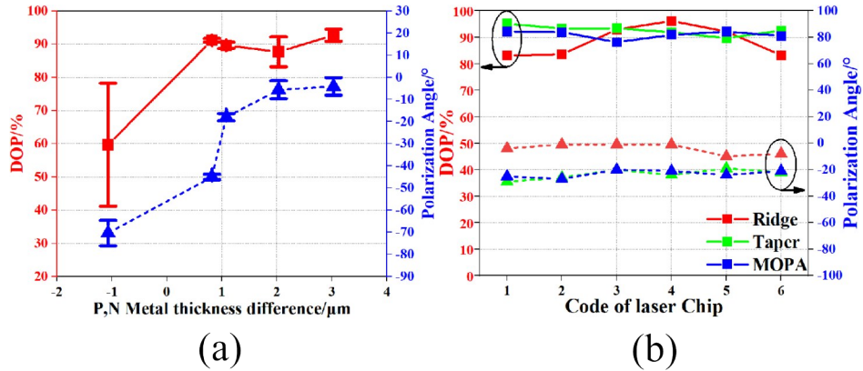
图4 (a)PN金属厚度差对MOPA偏振度、偏振角度的影响;(b)脊型、锥形、MOPA器件的偏振度与偏振角度 Fig. 4 (a) The influence of PN metal thickness difference on DOP and polarization angle of MOPA; (b) DOP and polarization angle of ridge, taper and MOPA
