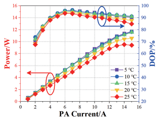
图6 MOPA器件的功率和偏振度随热沉温度的变化 Fig. 6 The impact of heat sink temperature on the power and DOP of MOPA device
