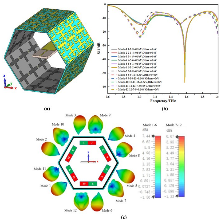
Fig. 6 Antenna characteristics of the loaded radome; (a) 3D Structure; (b) S-parameters in different modes; (c) radiation direction in different modes
