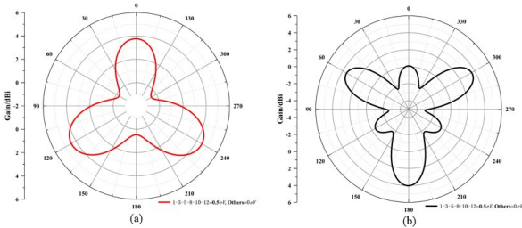
Fig. 8 Radiation direction when the interval between u_1 and u_2 is set to 0.5 eV 图8 u_1 和 u_2 间隔设置为0.5 eV时的辐射方向图
