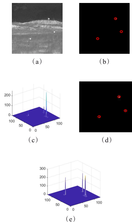
Fig.6 Comparison before and after nonlinear mapping: (a) original infrared image; (b) ADG; (c) 3D grayscale view of ADG; (d) \text{ADG}_{\text{mapped}}(x,y) ; (e) 3D grayscale view of \text{ADG}_{\text{mapped}}(x,y) 图6 非线性映射前后对比: (a)原始红外图像; (b) ADG; (c) ADG的三维灰度图; (d) \text{ADG}_{\text{mapped}}(x,y) ; (e) \text{ADG}_{\text{mapped}}(x,y) 的三维灰度图
