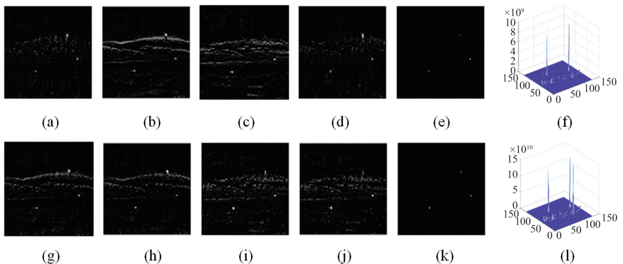
Fig.9 Comparison of associated directional gradient and single directional gradient: (a) left gradient; (b) upper gradient; (c) down gradient; (d) right direction; (e) single-direction gradient product; (f) mesh of (e), (g) left-upper gradient; (h) upper-right gradient; (i) down-left gradient; (j) right-down gradient; (k) associated directional gradient product; (l) mesh of (k)
