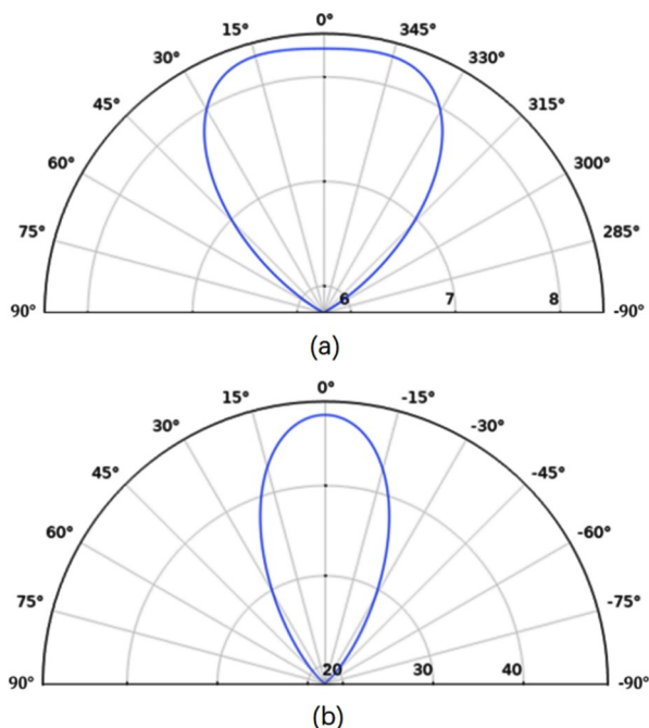
图6 远场强度分布:(a)无谐振腔,(b)有谐振腔 Fig. 6 The far field angular profile of the emission: (a) without the resonant cavity, (b) with the resonant cavity
