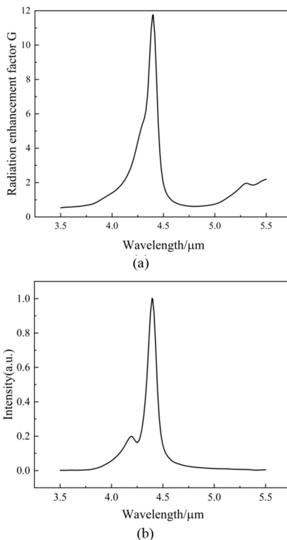
图7 (a)辐射增强因子G随波长的分布,(b)300 K时,RCLED的辐射光谱 Fig. 7 (a) The dependence of G on the wavelength, (b) the electroluminescence spectra of RCLED at 300 K
