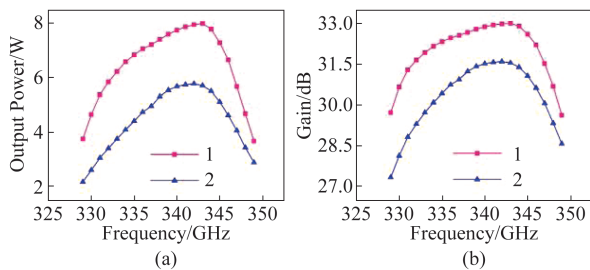
Fig. 16 Comparison of output between two structures (a) output power, and (b) gain Note: 1-with phase-velocity tapering, 2-without phase-velocity tapering 图16 两种慢波结构的比较(a)输出功率,(b)增益 注:1-使用相速调度技术,2-不使用相速调度技术
