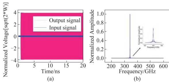
Fig. 13 Output (a) signal, and (b) frequency spectrum 图 13 (a)输出信号波形,(b)输出信号频谱
