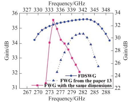
Fig. 17 Comparison of operating frequency and bandwidth 图17 工作频带和带宽的比较
