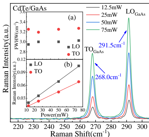
图4 不同激发功率的CdTe/GaAs薄膜FT红外拉曼光谱。插图为FWHM(a)和拉曼强度(b)随激发功率的演变规律 Fig. 4 FT infrared Raman spectra of CdTe/GaAs thin film at different excitation power. Inset: evolutions of FWHM(a) and Raman Intensity(b) with excitation power
