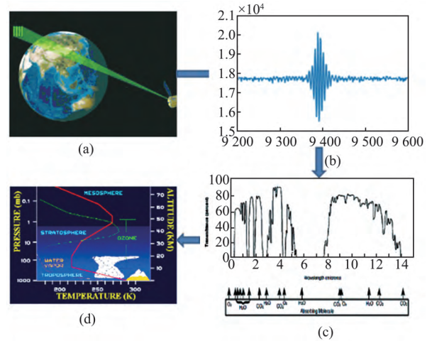
Fig. 2 Flow chart for information transformation of atmospheric vertical sounder ( a ) Measurement model of atmospheric vertical sounder ( b ) Interference signal ( c ) Radiation spectrum , ( d ) Vertical detection
