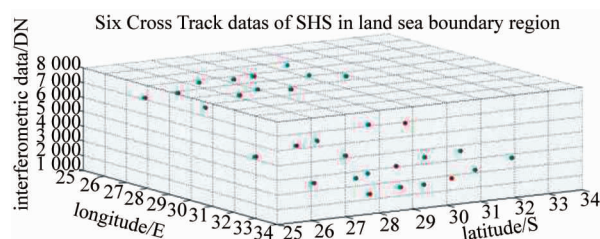
图 8 海岸区域内穿轨方向 SHS 各个观测点实际指向位置 (红点) 和参考指向位置 (绿点) 以及干涉数据值分布 Fig.8 The distributing of pointing location (red) and reference pointing location (green) and the interferometric data of many targets on earth in cross track measured by SHS in the land-sea boundary region
